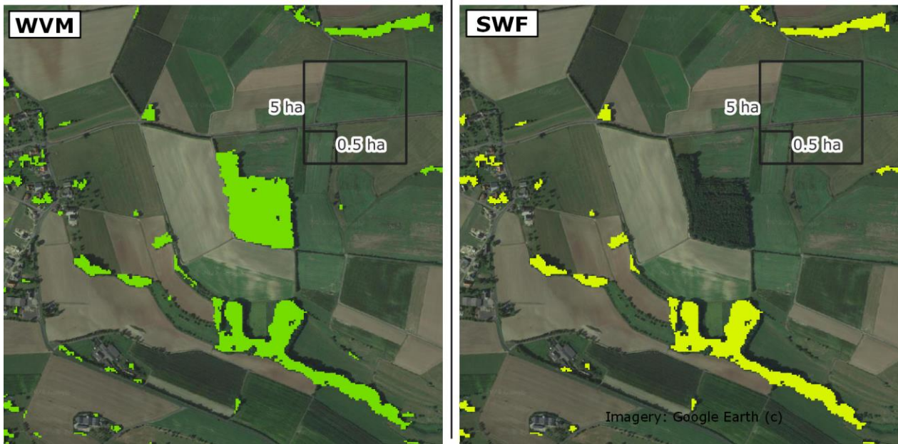
Figure 15 Comparison of WVM (l), SWF (r). Patch in the centre of the image, as well as small linear patches (West) were removed from SWF layer due to size restriction. (WGS 84: 50.041, 6.454).
